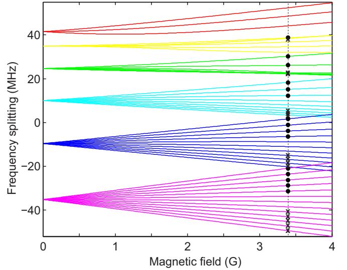
FIG. 2. (Color online) Hyperfine and Zeeman splitting of the D_{5/2} state manifold calculated for hyperfine constants measured in our experiment. Filled circles (●) and crosses (×) mark states that can be excited starting from the S_{1/2}(F=4) state with magnetic quantum number m_F=+4 ( m_F=-4 ), respectively. The vertical dashed line indicates the magnetic field used for measuring the frequency shifts in the experiment.
