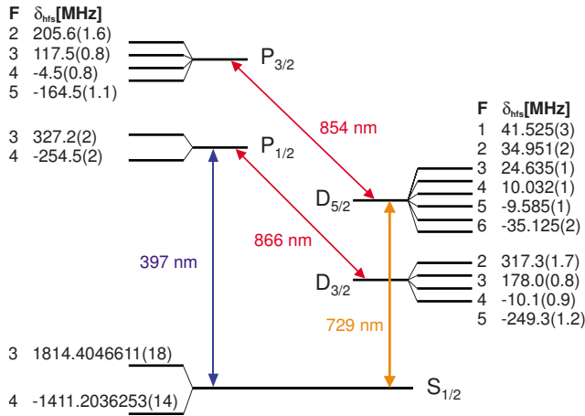
FIG. 1. (Color online) ^{43}\text{Ca}^+ level scheme showing the hyperfine splitting of the lowest energy levels. Hyperfine shifts \delta_{\text{hfs}} of the levels are quoted in MHz (the splittings are taken from [10,11] and our own measurement). Laser light at 397 nm is used for Doppler cooling and detection; the lasers at 866 and 854 nm pump into the D states. An ultrastable laser at 729 nm is used for spectroscopy on the quadrupole transition.
