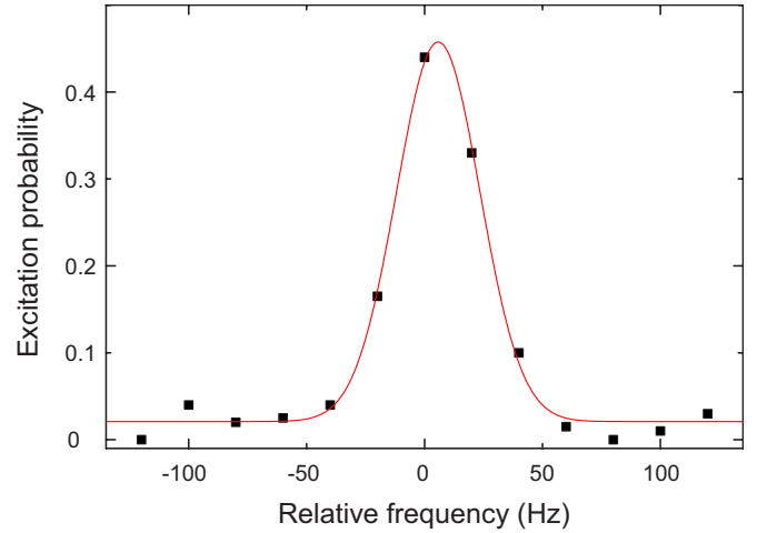
FIG. 4. (Color online) Frequency scan over the transition S_{1/2}(F=4, m_F=4) \leftrightarrow D_{5/2}(F=4, m_{F'}=3) with an interrogation time of 100 ms. A Gaussian fit (solid line) determines a width of 42 Hz which is dominated by the linewidth of the spectroscopy laser at 729 nm.
