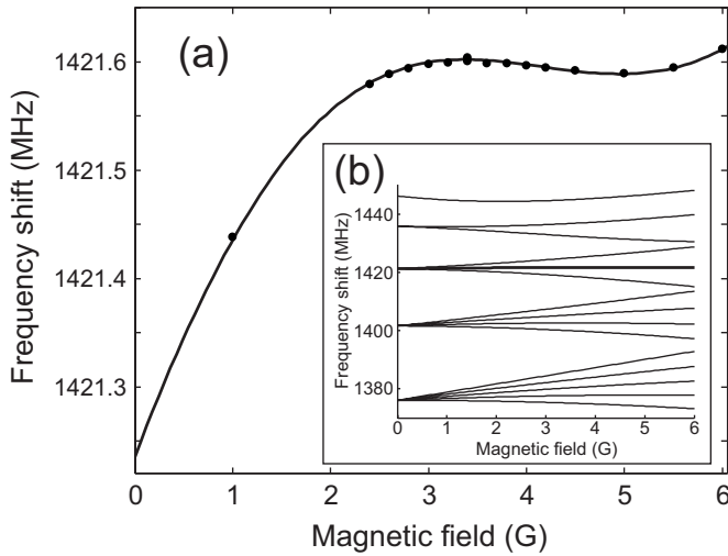
FIG. 3. (a) Frequency dependence of the S_{1/2}(F=4, m_F=4) \leftrightarrow D_{5/2}(F=4, m_F=3) transition frequency for low magnetic fields. The transition frequency becomes field-independent at B=3.38 G and B=4.96 G with a second-order Zeeman shift of \pm 16 kHz/G 2 . The measured data are not corrected for the drift of the reference cavity which may lead to errors in the shift of about 1–2 kHz. To match the data with the theoretical curve based on the previously measured values of A_{D_{5/2}} and B_{D_{5/2}} , an overall frequency offset was adjusted. (b) Calculated shift of the fifteen allowed transitions starting from S_{1/2}(F=4, m_F=4) . The thick line shows the transition to the state D_{5/2}(F=4, m_{F'}=3) .
